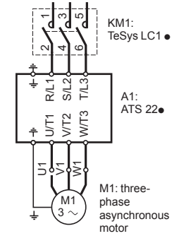
Motor starter with protection by circuit breaker or switch disconnector
