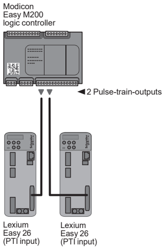
Example of architecture with control by Modicon Easy M200 logic controller
